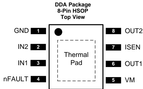
Pin Functions
